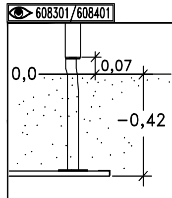
SF Sunken Foundation 8096533
